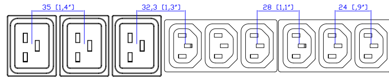
VIEW B
