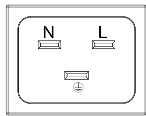
IEC320 C20
