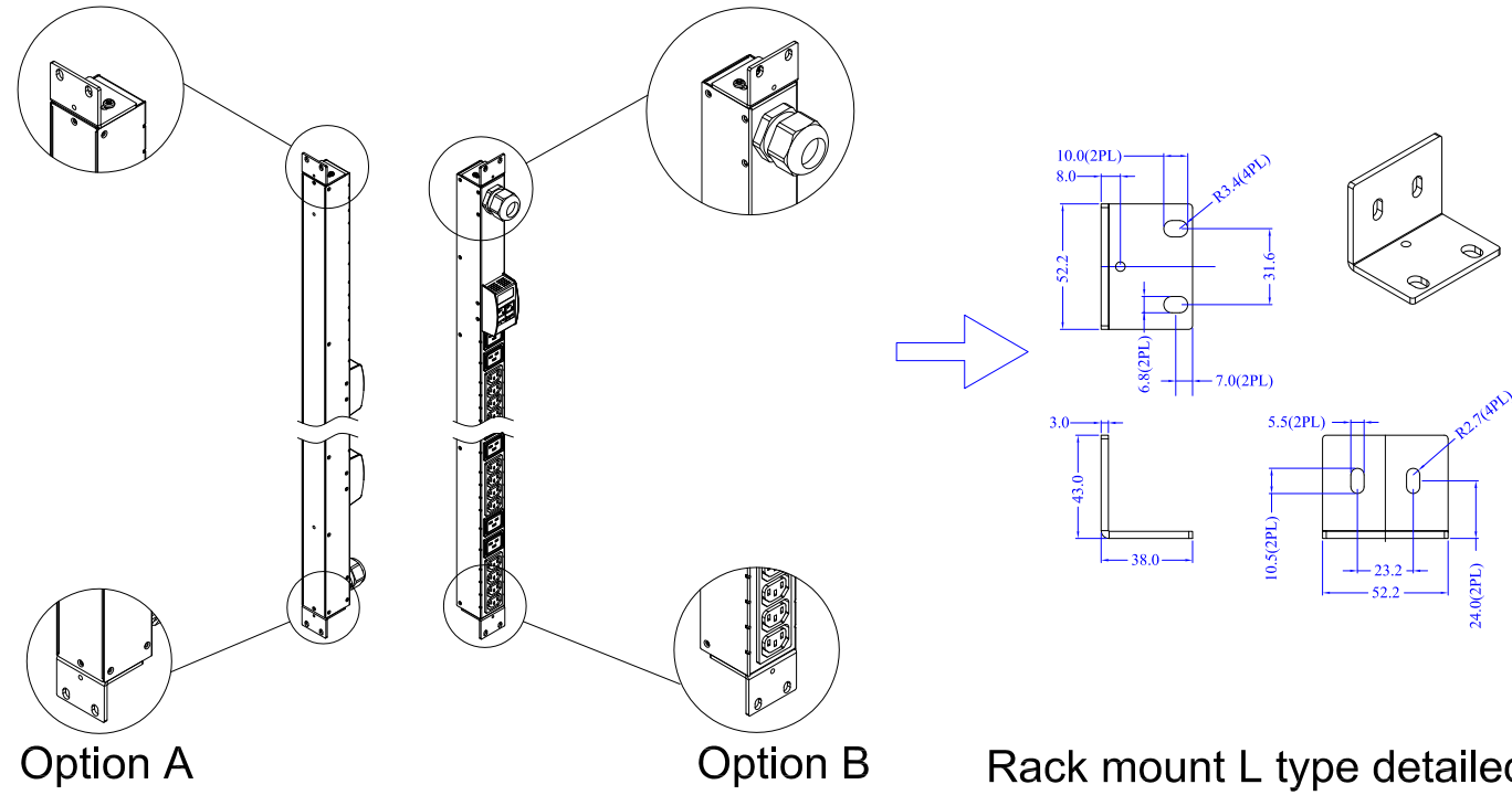
Mounting options
