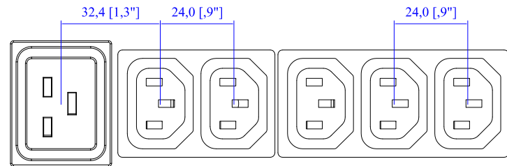
VIEW A
