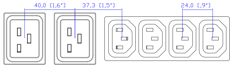
VIEW B
