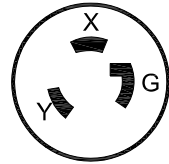
NEMA L6-30P VIEW A
