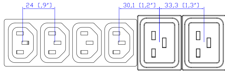
VIEW B
