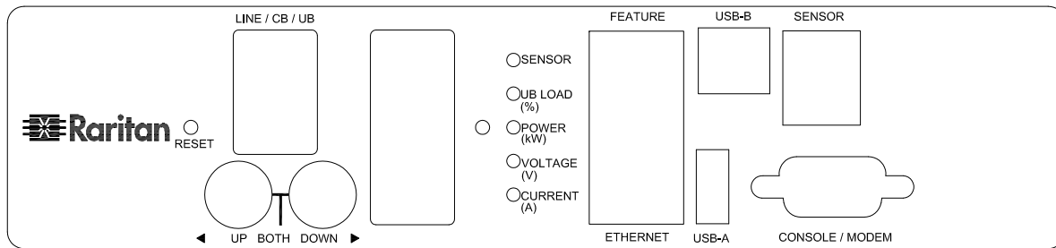
VIEW C
