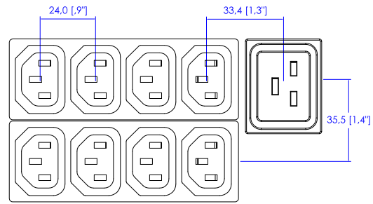
VIEW B
