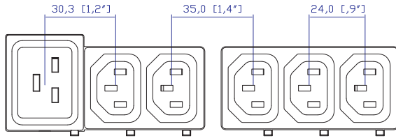
VIEW B
