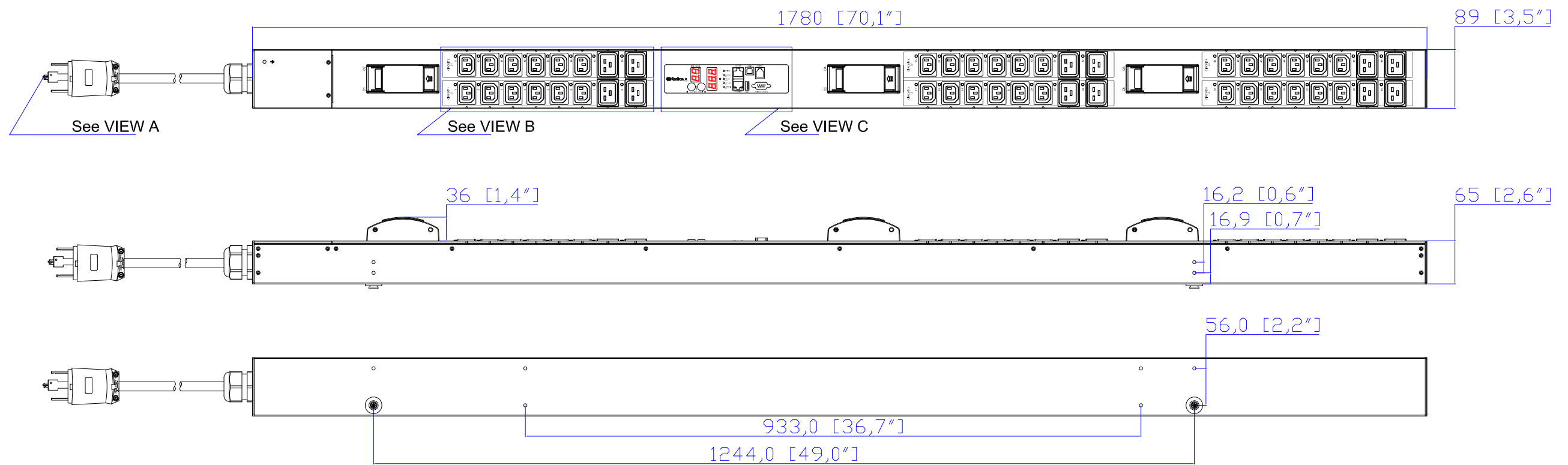
VIEW C
