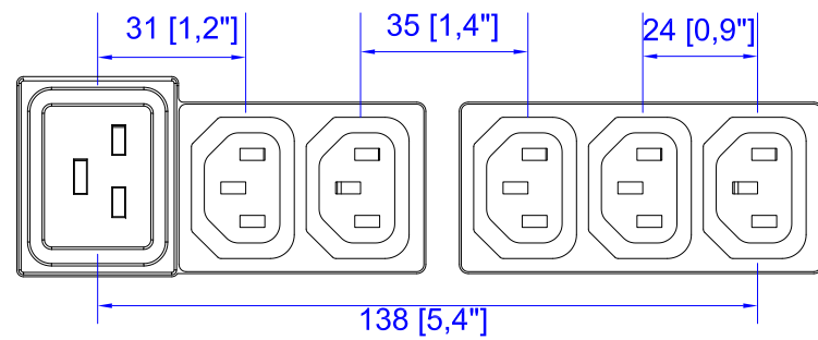
VIEW B
