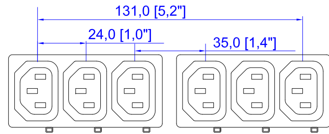
VIEW A
