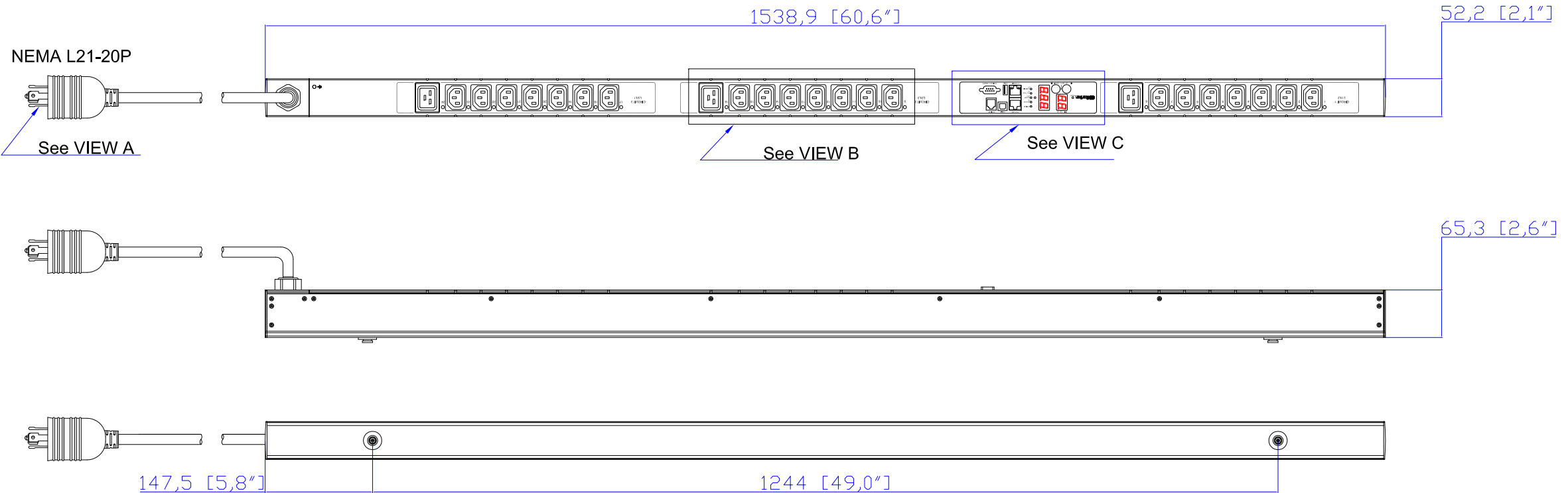
VIEW C
