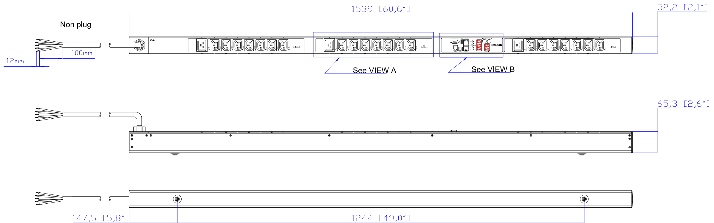
VIEW B
