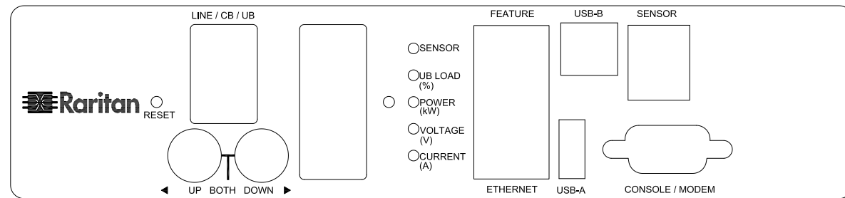
VIEW A
