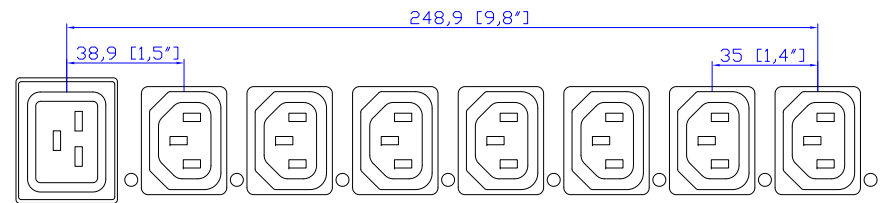
VIEW A
