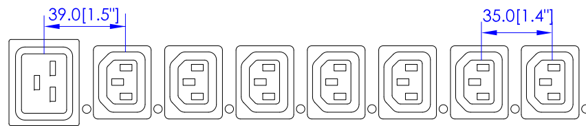
VIEW B
