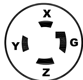
VIEW A
