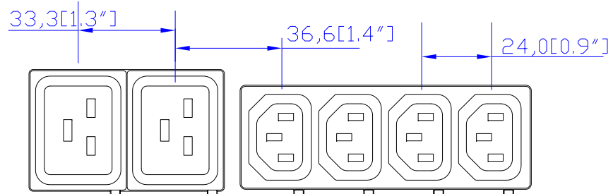
VIEW B
