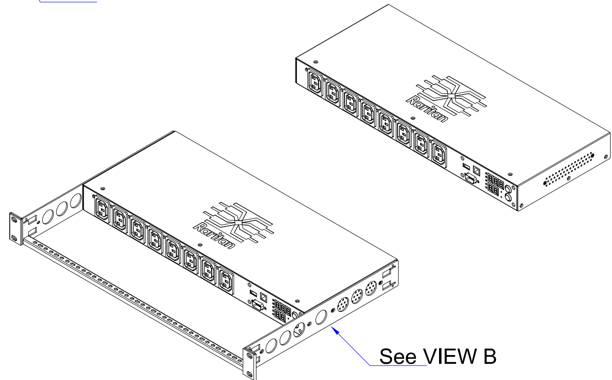
VIEW C
