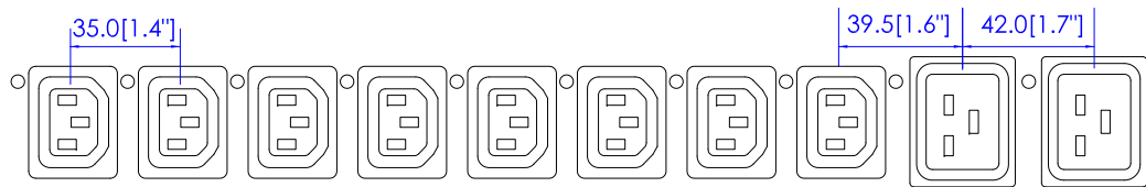
VIEW A
