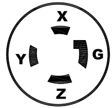
VIEW A
