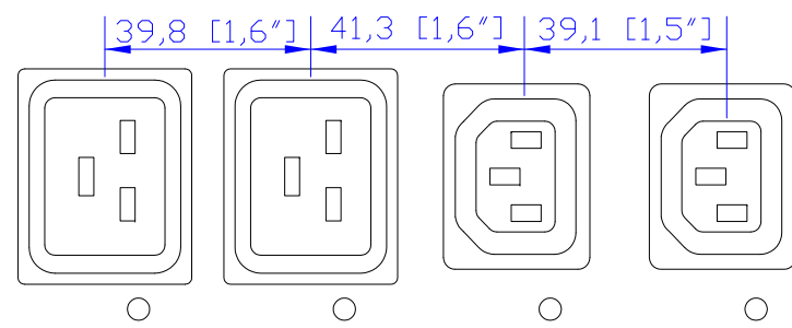
VIEW B
