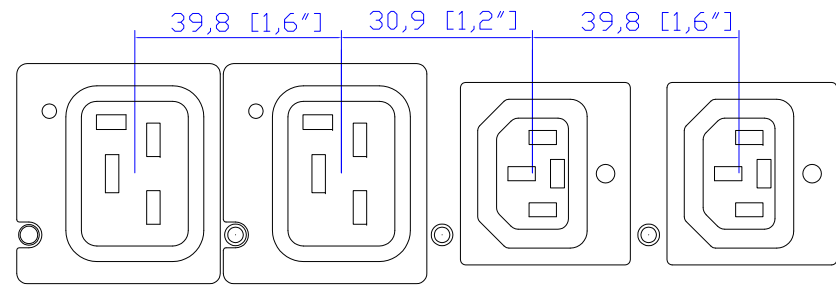
VIEW A
