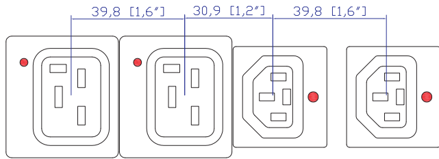
VIEW A
