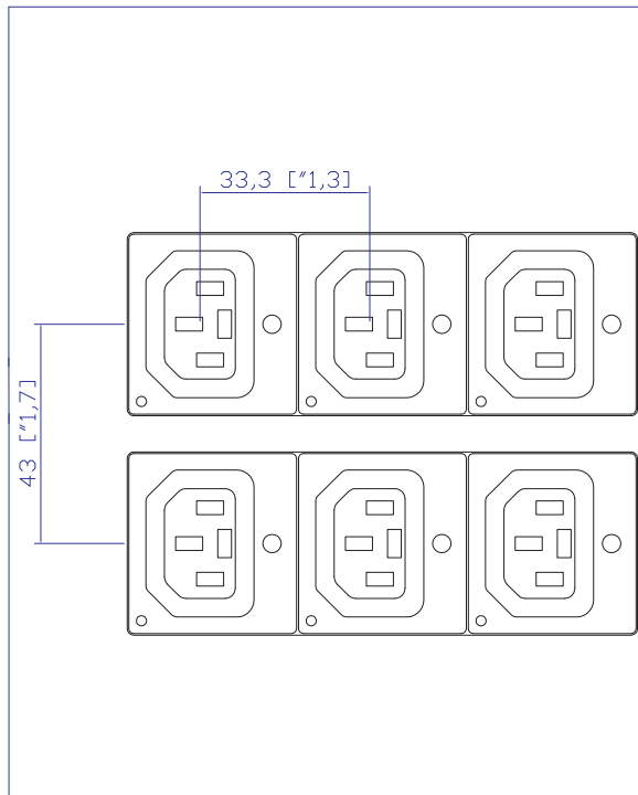
VIEW A
