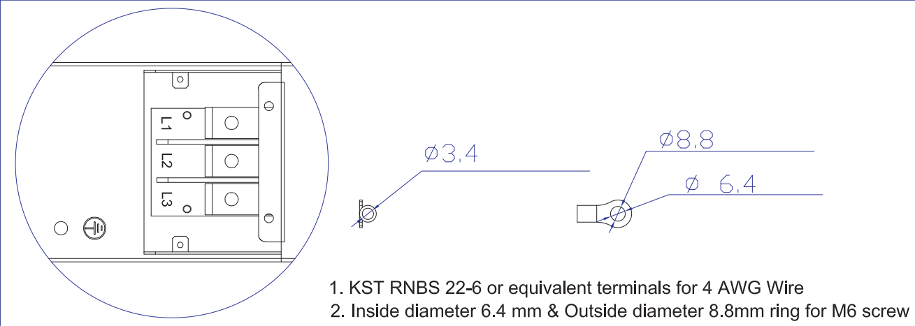
VIEW C
