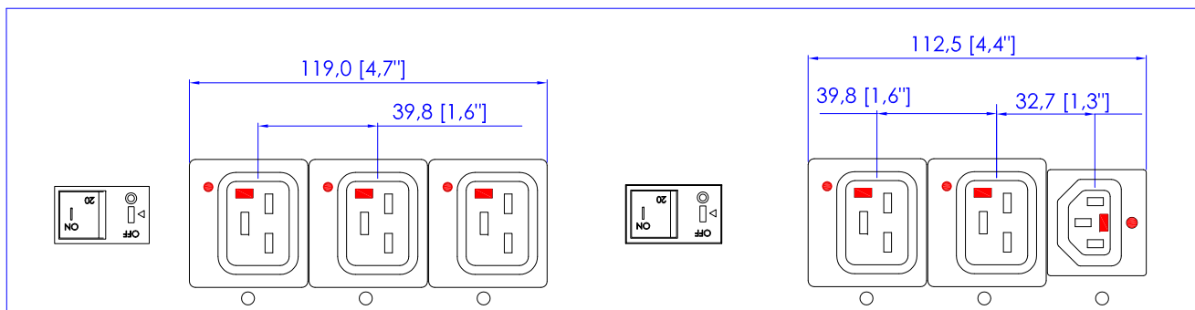
VIEW A
