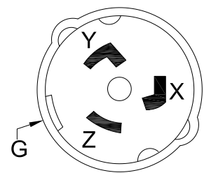
CS8365C VIEW A
