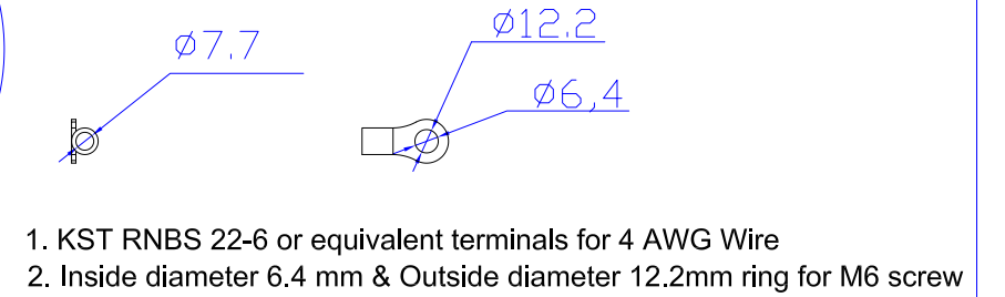
VIEW C
