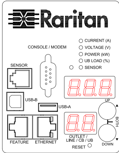
VIEW A
