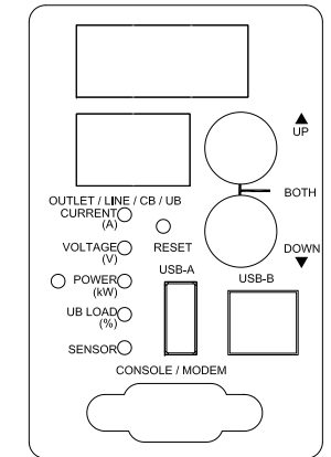
VIEW C
