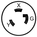
NEMA L6-30P VIEW A
