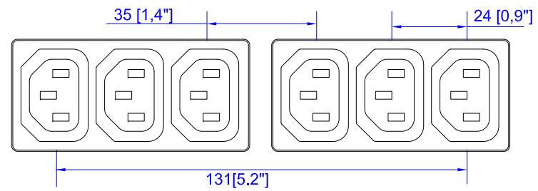
VIEW B
