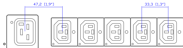
VIEW B
