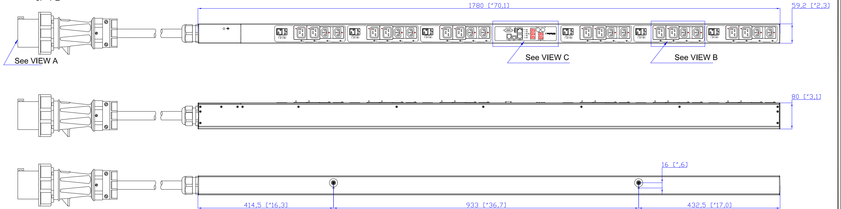
IEC309 60A/250V 3P+PE
