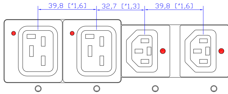
VIEW B
