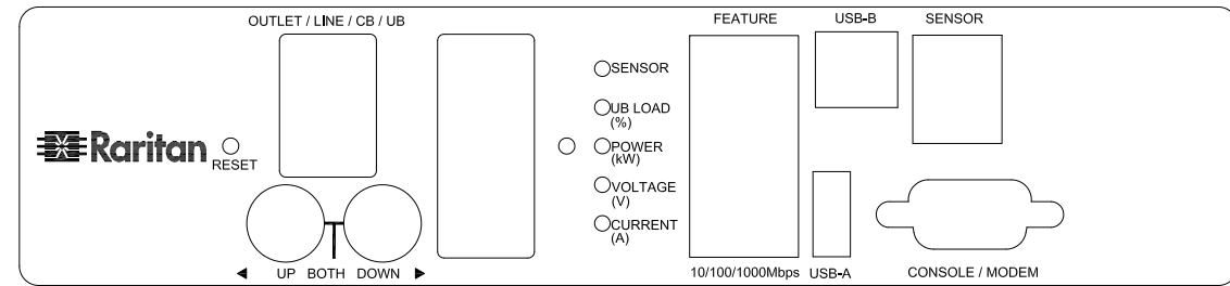
VIEW C
