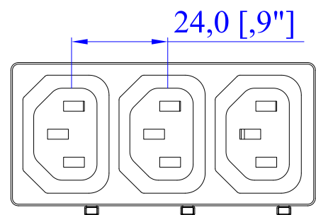
VIEW B
