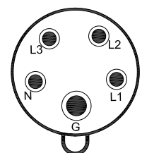
IEC309 32A/400V 3P+N+PE
