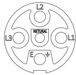
Clipsal 56P532
