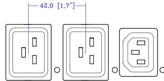
VIEW B
