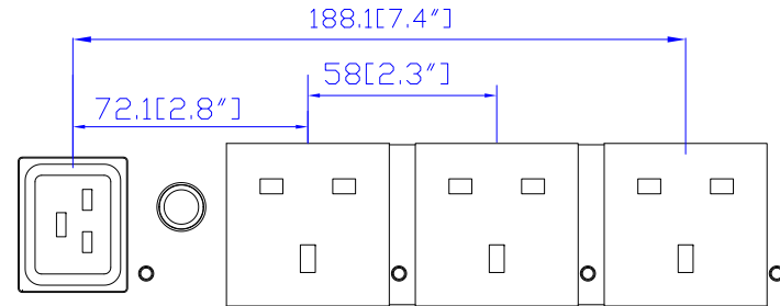
VIEW B
