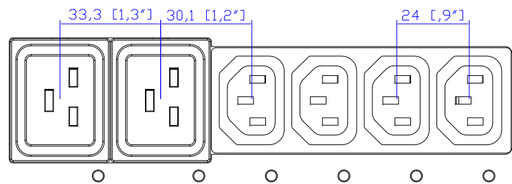
VIEW B
