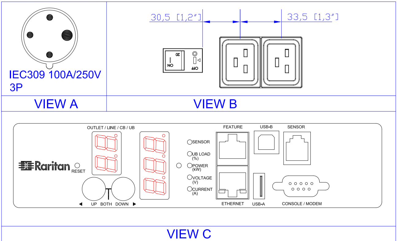
IEC309 100A/250V 3P
