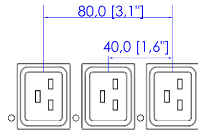
VIEW B
