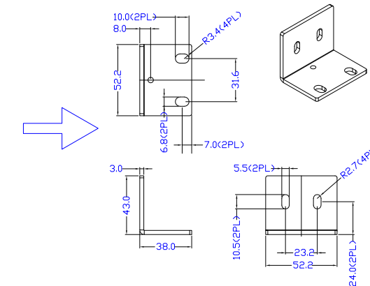
Rack mount L type detailed
