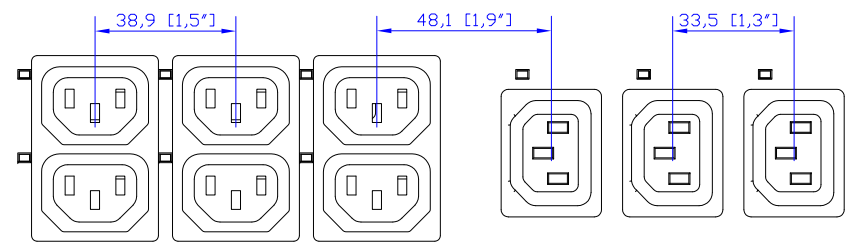
VIEW A
