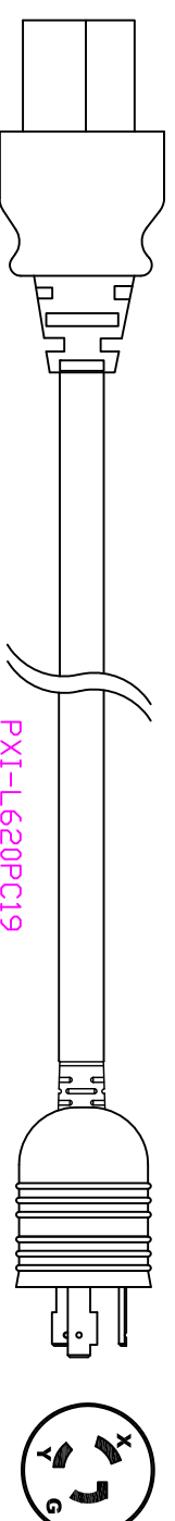
IEC60320 C19
