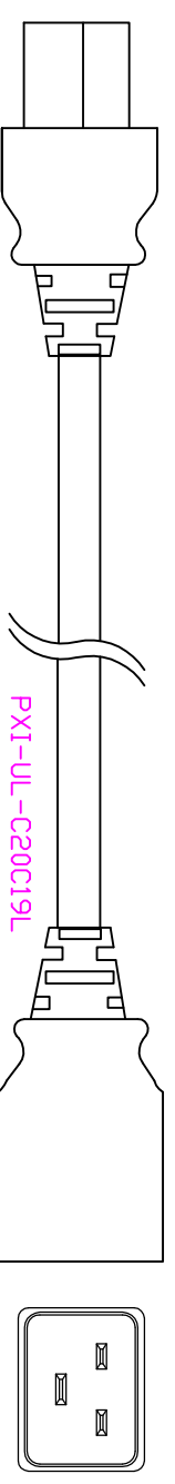
IEC60320 C19
