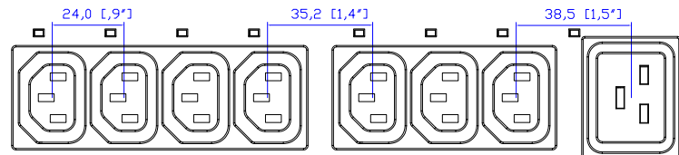
VIEW B
