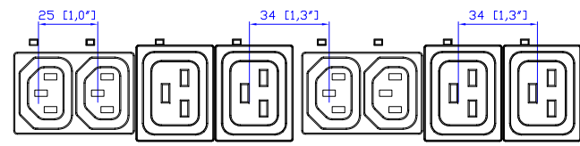
VIEW B
