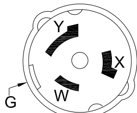
CS8365C VIEW A
