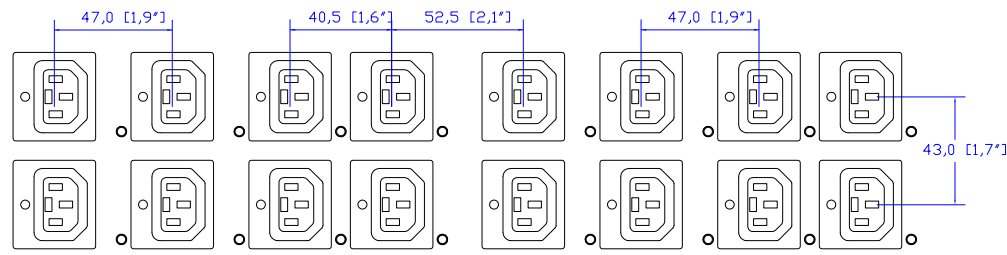
VIEW A
