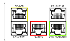
VIEW B
