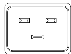
IEC60320 C20
